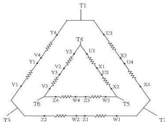
SCHEMATIC - 2Δ / Δ CONNECTION
