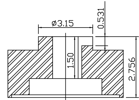
Coupling Dimension
