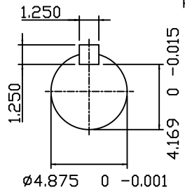
SHAFT END (ENLARGED VIEW)
