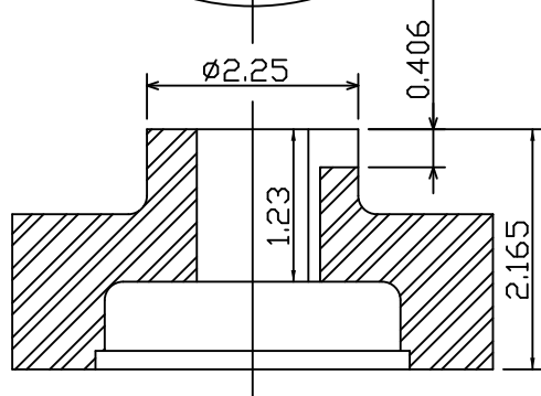
Coupling Dimension
