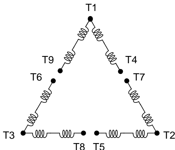
SCHEMATIC — 2△/△ CONNECTION
